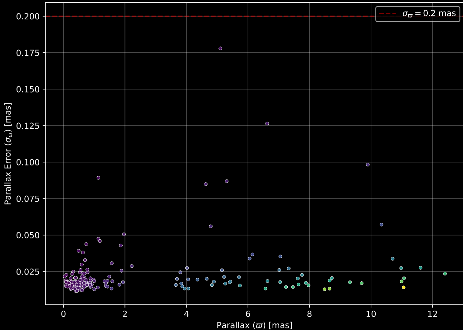
APOGEE DR17 Field: [198+24_MGA] Parallax Quality (n= 178)
