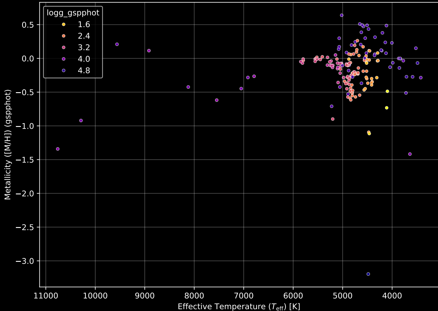
APOGEE DR17 Field: [198+24_MGA] Stellar Population Parameters (n= 178)
