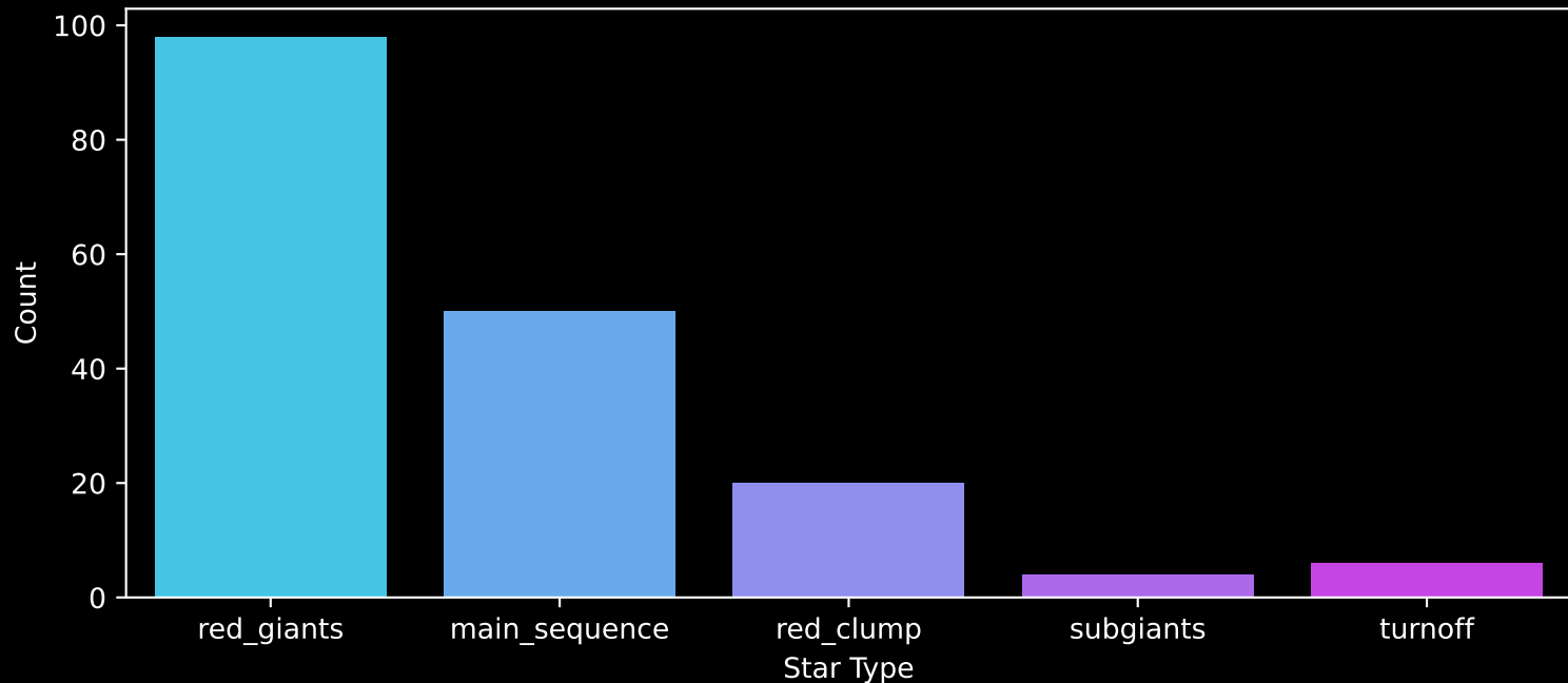
APOGEE DR17 Field: [198+24_MGA] Count plot of Star Type
