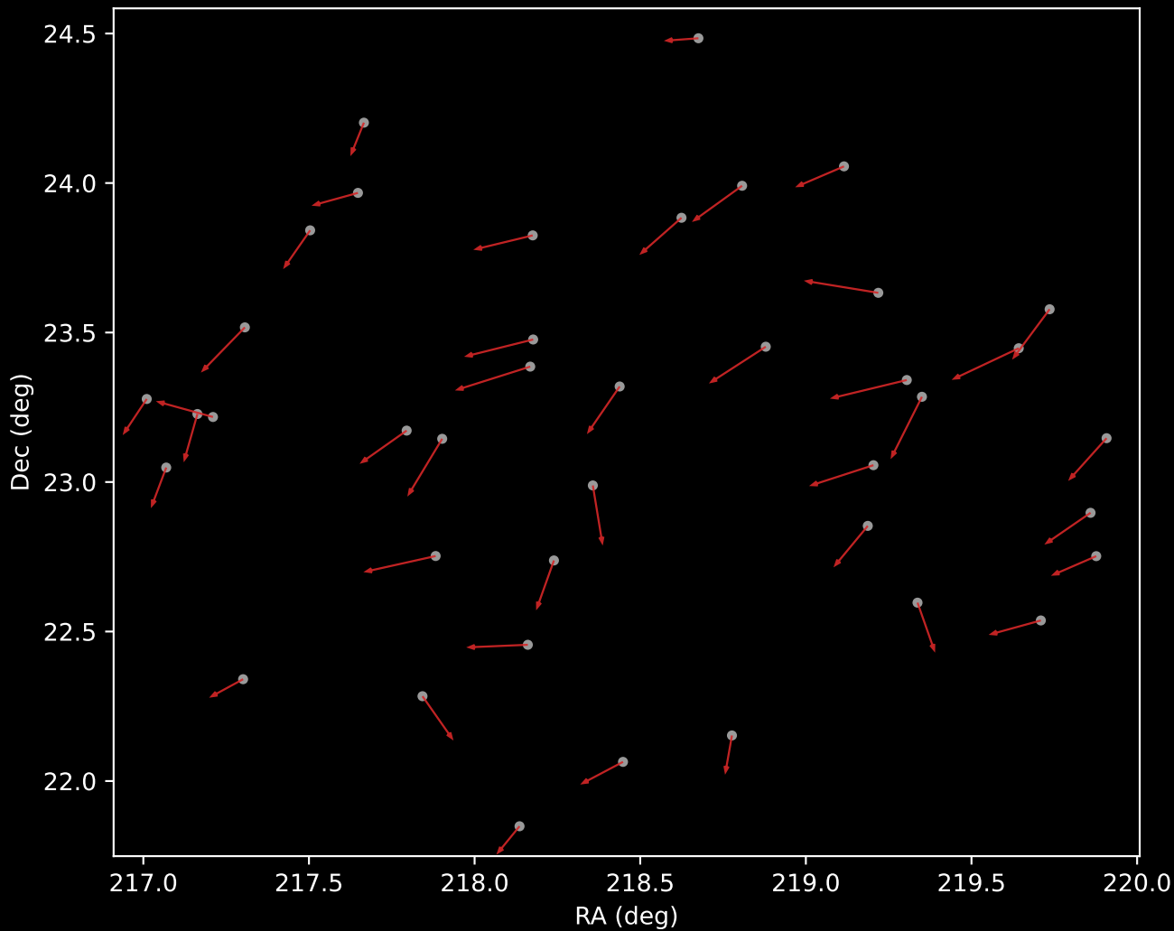
APOGEE DR17 Cluster 6 Proper Motion Vectors (n=40)
