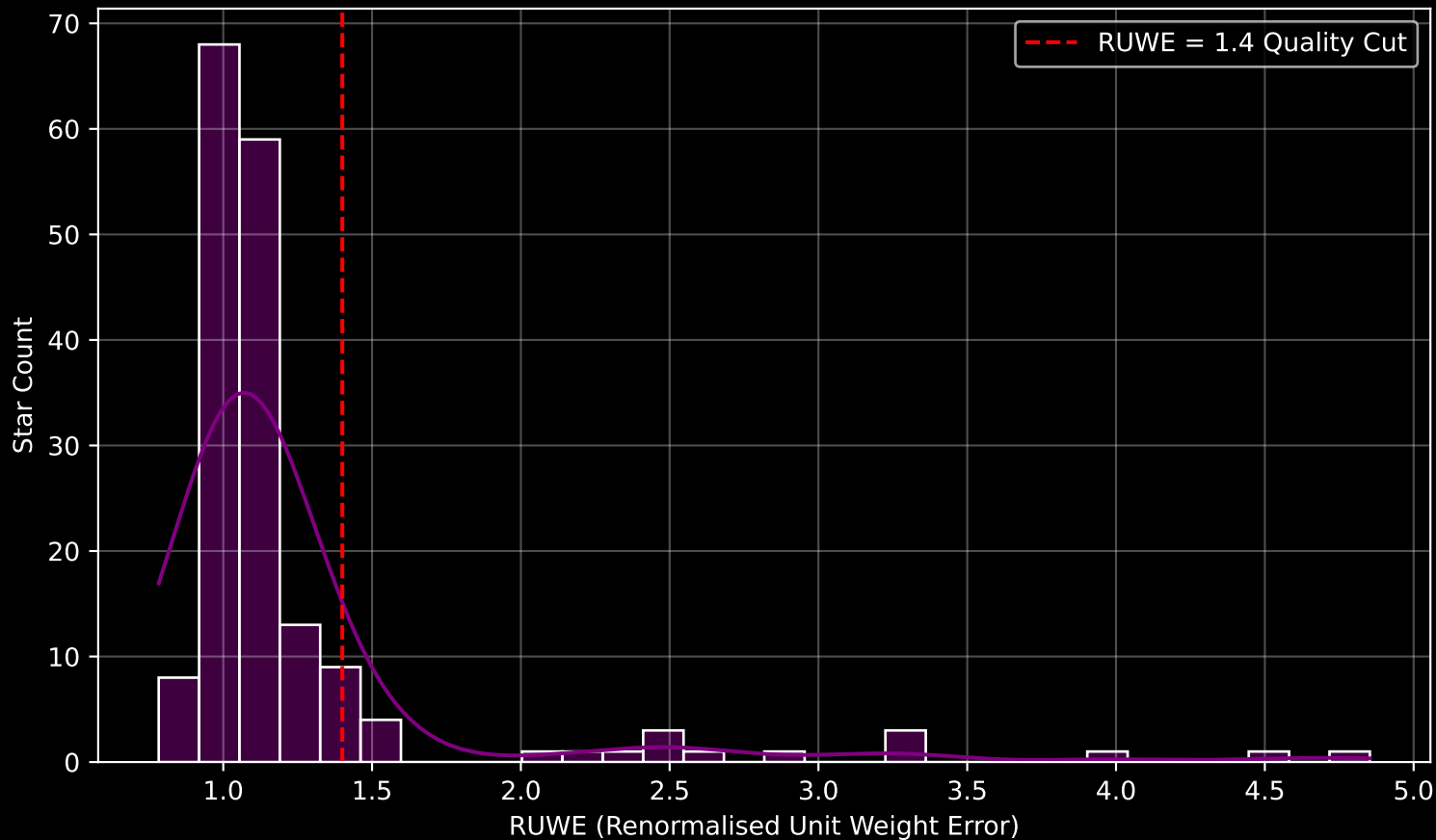
GAPOGEE DR17 Field [198+24_MGA] RUWE Distribution (n= 175)
