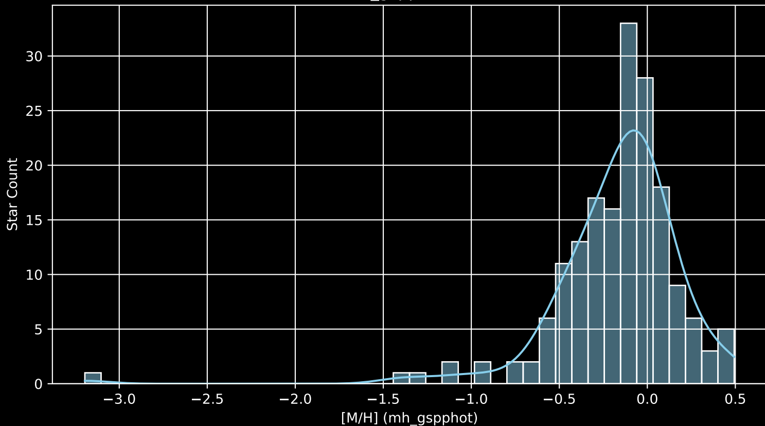
APOGEE DR17 Field: [198+24_MGA [M/H] (mh_gspphot) (n= 176)
