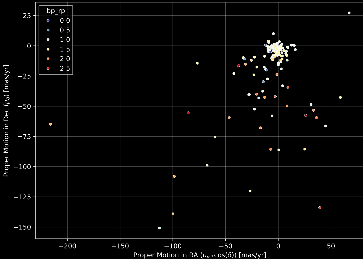
APOGEE DR17 Field: [198+24_MGA] Proper Motion Diagram (n= 178)
